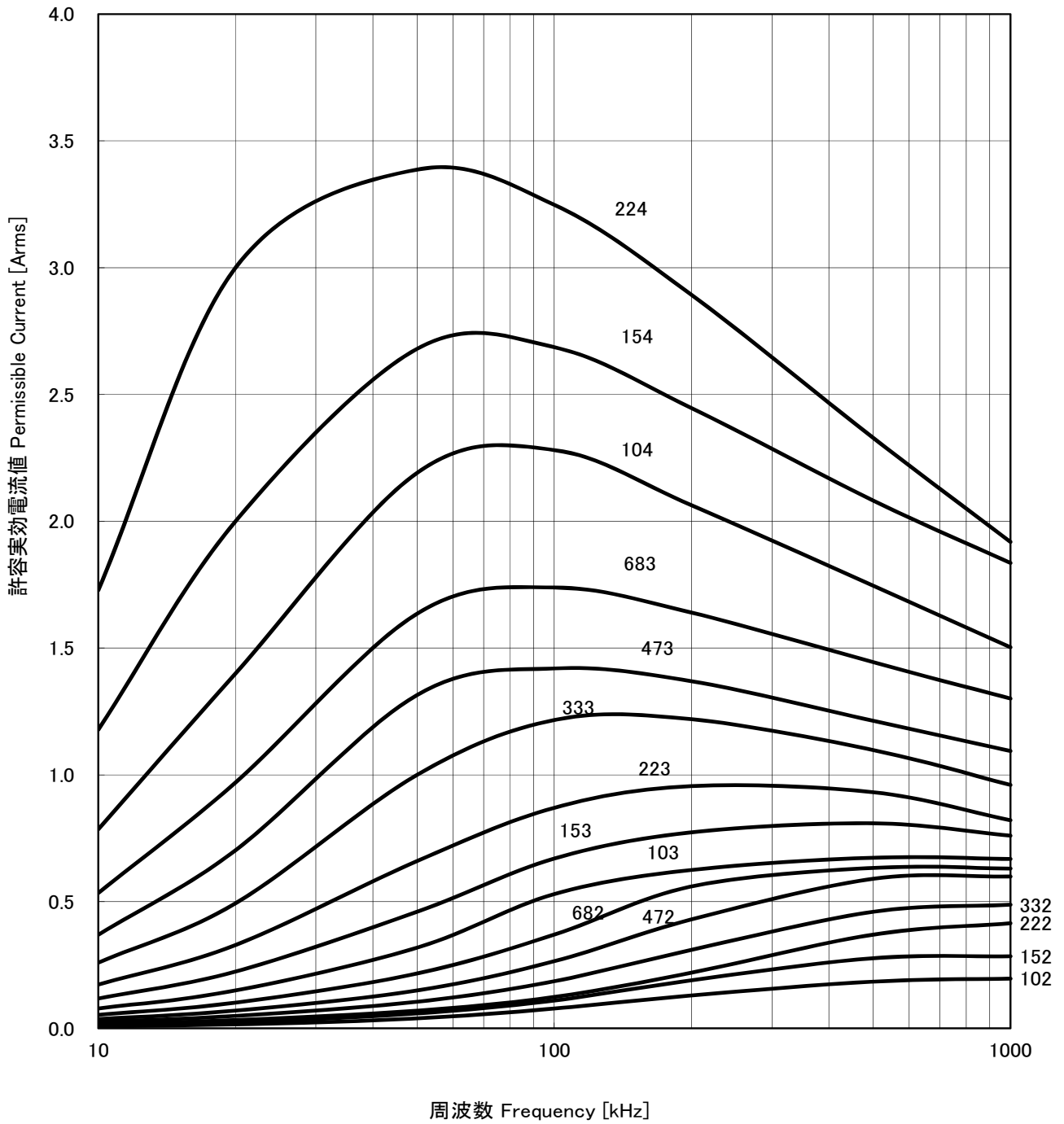
周波数別許容実効電流値 FPB 1250VDC Permissible Current vs Frequency
